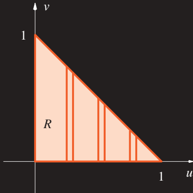
Figure 7.29 The integration region R in Example 4.
